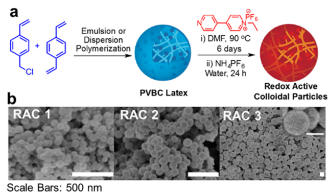
Figure 1. Synthesis and SEM images of redox active colloidal particles (RACs). (a) Reaction scheme for the synthesis of polyvinyl benzyl chloride and viologen based redox active colloidal particles. (b) SEM images of the fully substituted viologen RACs 1–3 in the dry state: particle diameters of 80 \pm 11 , 135 \pm 12 , and 827 \pm 71 nm, respectively. Scale bar: 500 nm.
