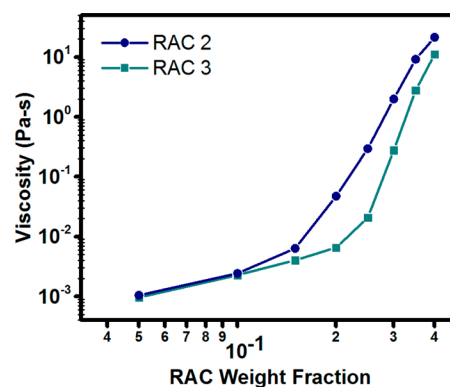
Figure 6. Rheological properties of RACs. Apparent viscosity measured at 100 s -1 of viologen dispersions of varying particle size and weight fraction in acetonitrile with 1 M LiBF_4 .
